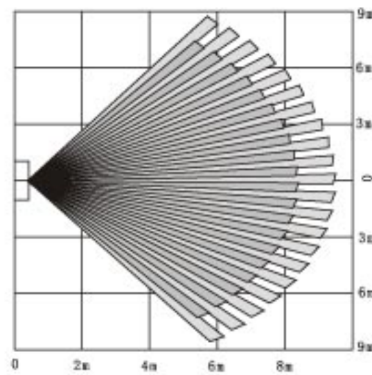
Wall mounting wide angle lens view
